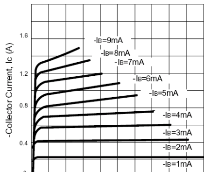
Static Characteristics
