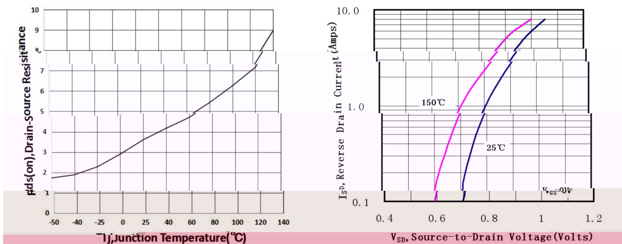
Fig3 Nonlinear Drain Resistance vs. Temperature Fig4 typical source-drain Diode Forward Voltage
